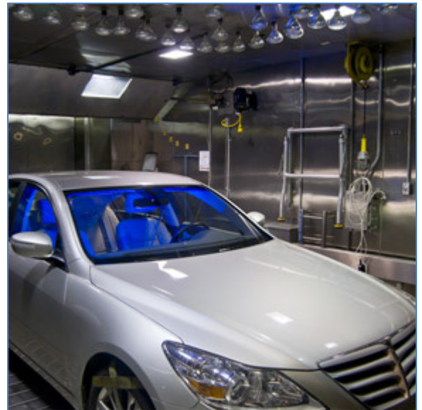
Typical chamber set-up for Environmental Vehicle Testing Laboratory at Delphi's Technical Center Rochester
